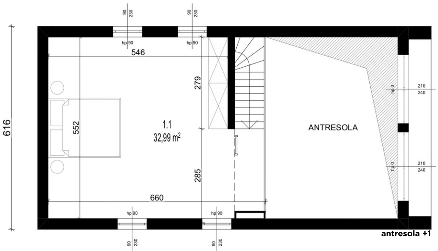
1.1 ANTRESOLA +1
